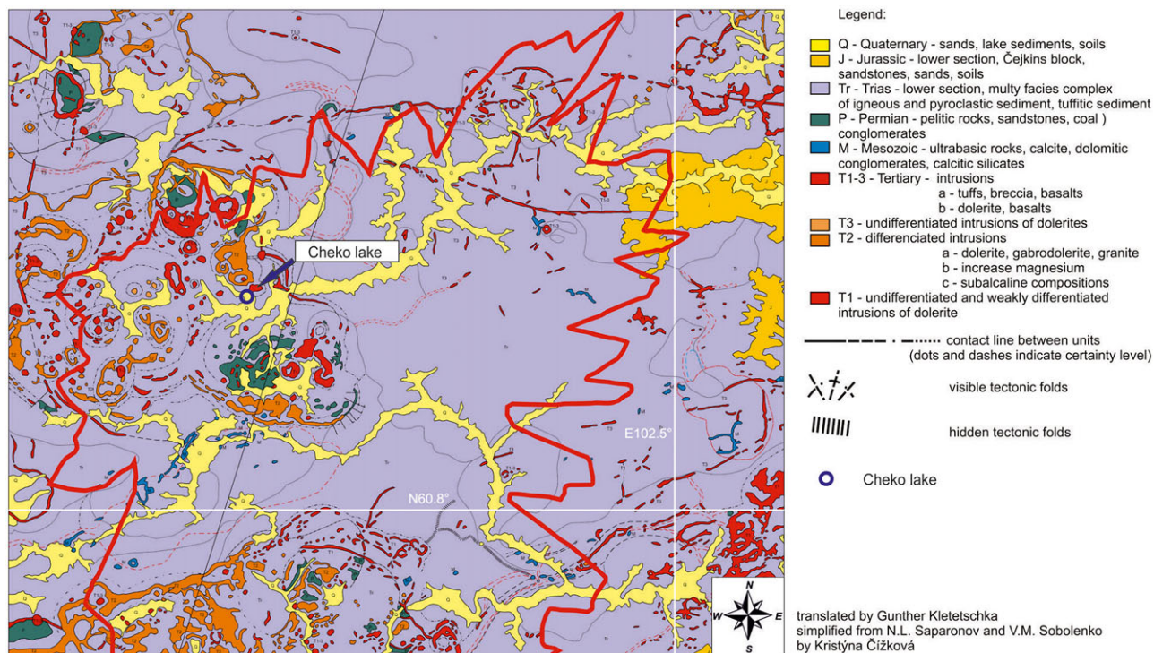
Fig. 3. Geological map of Cheko Lake.
