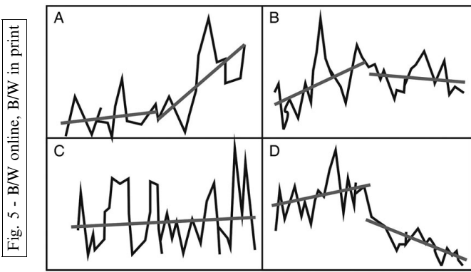
Fig. 5. Four classes of BAI: (A) young tree or not dominated anymore; (B) mature tree in closed space or with strong competition; (C) mature tree; (D) decline tree (adapted from Le Blanc, 1996).
