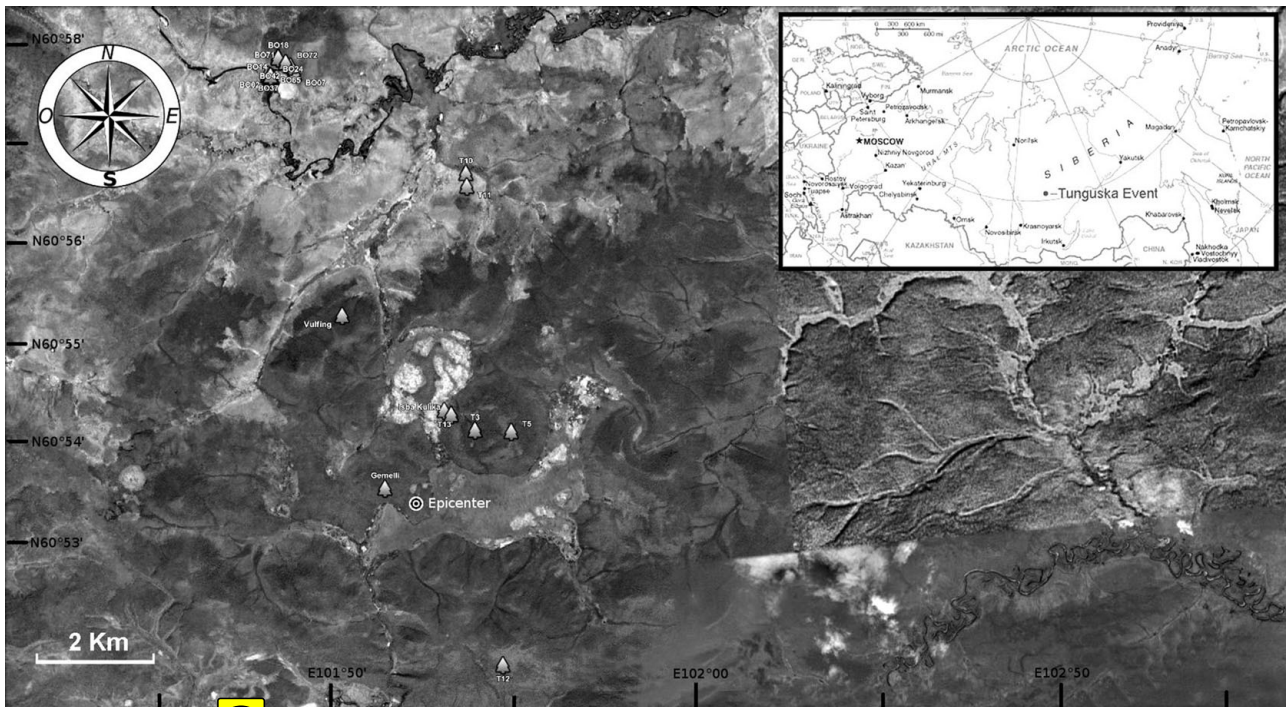
Fig. 2. Satellite map of the Tunguska area.
